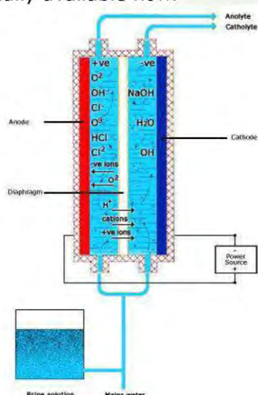
Design of Envirolyte cell
